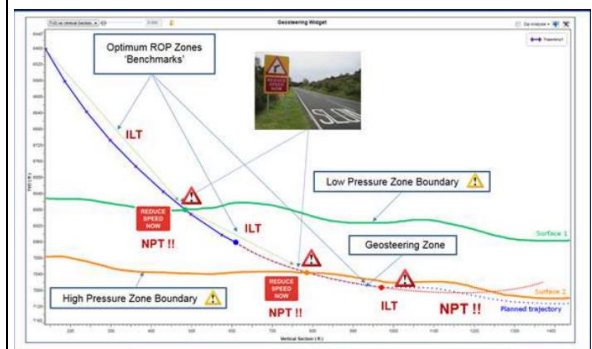
Figure #8: Link between drilling data and subsurface earth model (Curtis, 2018)
