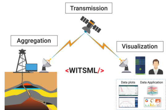
Figure #2: Real-time data flow from the rig to the monitoring specialist
